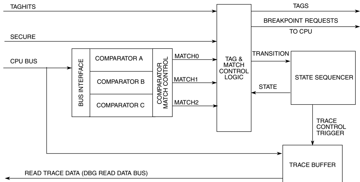
Figure 8-23. DBG Overview
