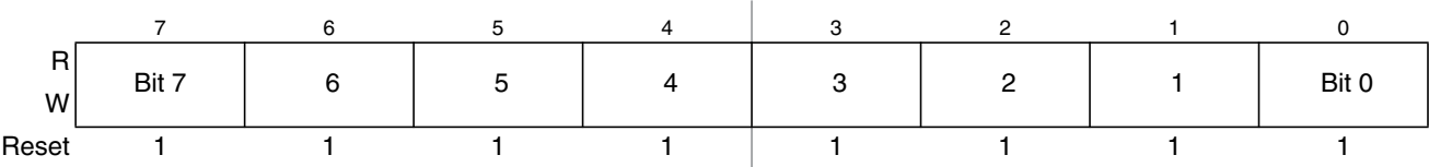
Figure 19-13. PWM Channel Period Registers (PWMPERx)
