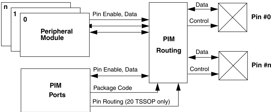
Figure 2-1. Block Diagram
