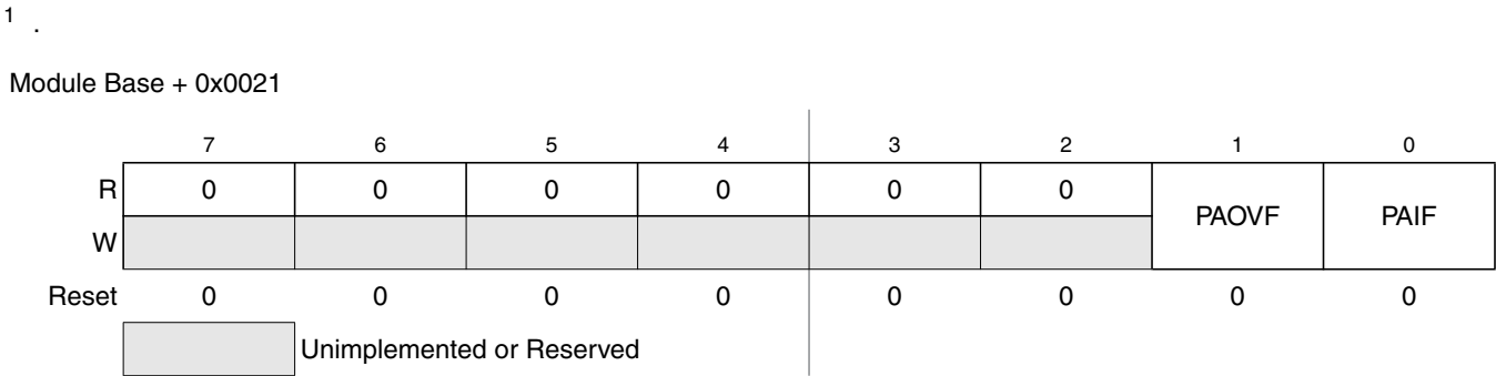
Figure 23-25. Pulse Accumulator Flag Register (PAFLG)
